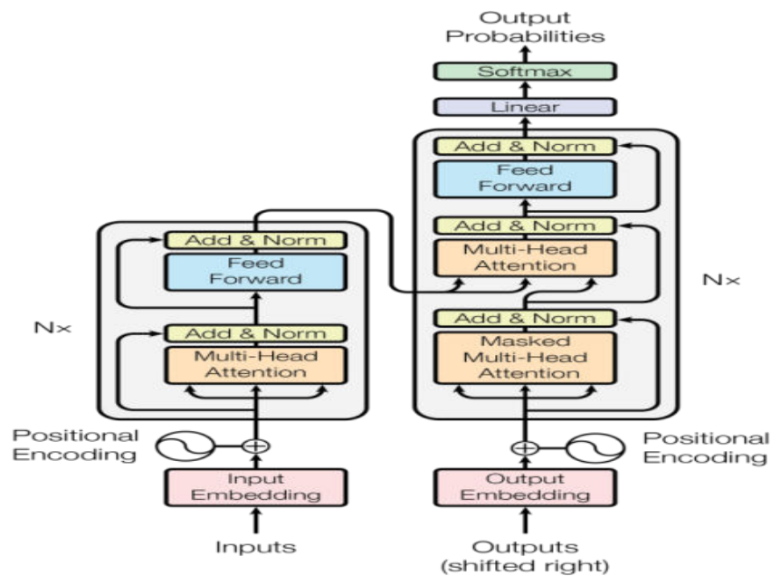
Fig 1: Transformer Architecture Overview
